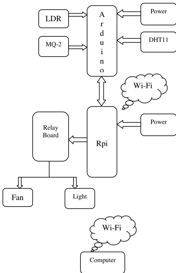
Fig. 1 Block Diagram
